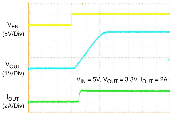
Time (500μs/Div)
