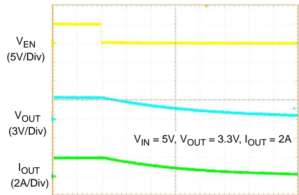
Time (10μs/Div)
