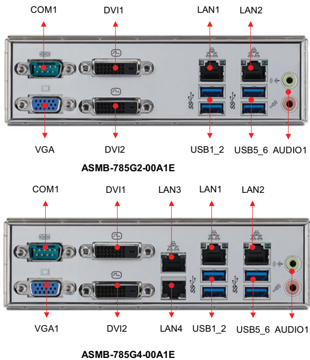
Figure 1.2 I/O connectors
